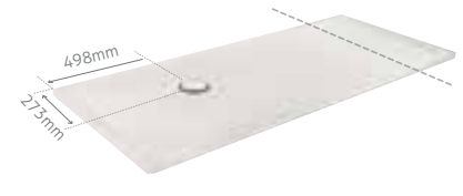
Size: 1700 x 750mm Code: SL3517075/CWEC (Can be cut to length. End cap supplied)
