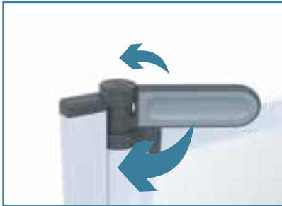
Paddle rotates 90° to lift the doors clear of the floor
