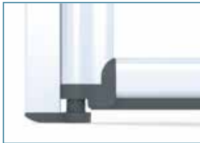
When the door is opened, the Elevate door rises to create a 15mm gap. This is from the bottom of the seal to the top of the shower tray or vinyl floor
